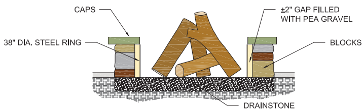
CROSS-SECTION
