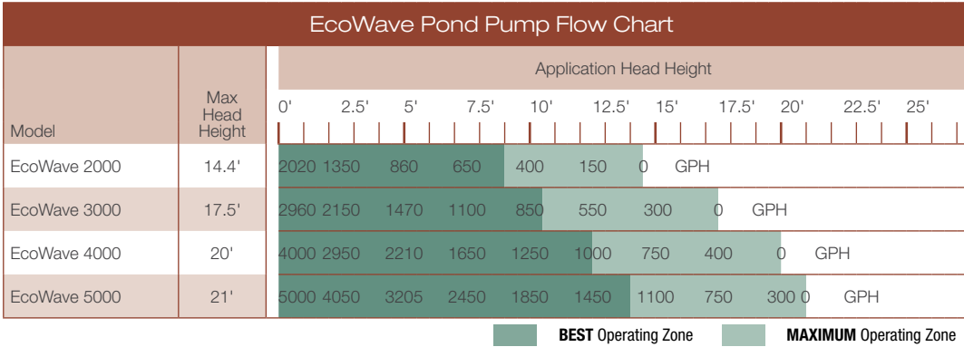
EcoWave Pond Pump Pipe Diameter Chart
