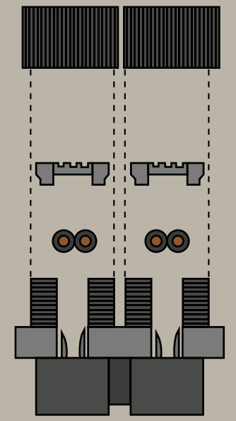
FRONT VIEW CABLE CONNECTOR CC-2
